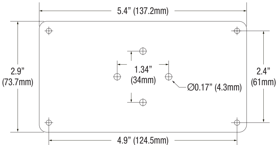
DNP1 Vertical mounting (front view)
